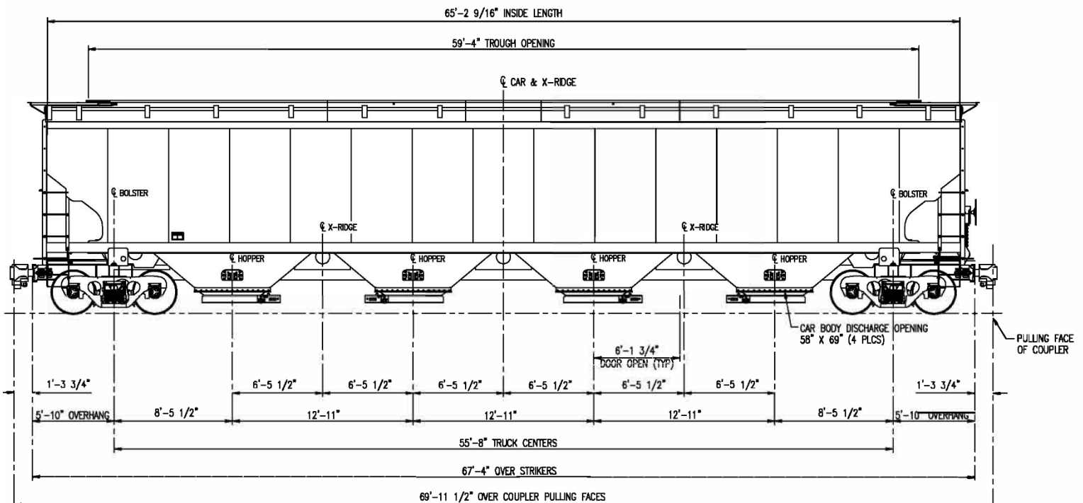
SIDE VIEW
